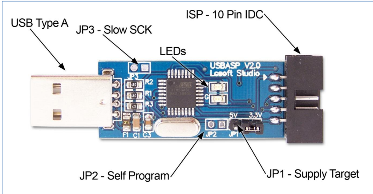
Figure 1. Device Layout
