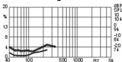
Distortion - Magnitude
