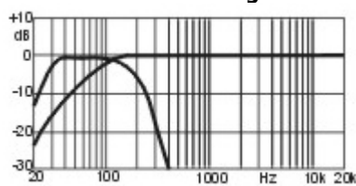
Combination - Magnitude
