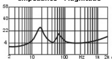
Impedance - Magnitude
