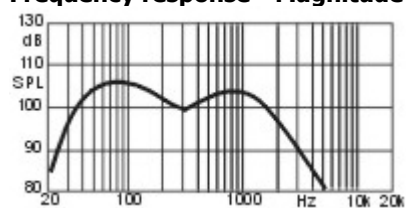
Frequency response - Magnitude
