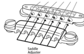
Intonation adjustment screw (for each string)
