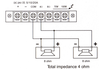
Connecting the speakers to 4 ohm output
