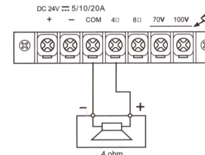
Connecting the speakers to 4 ohm output
