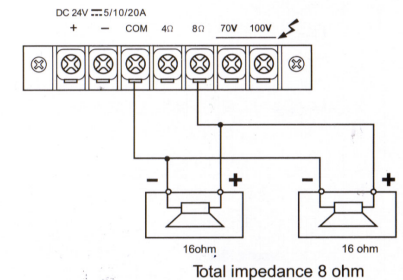
Connecting the speakers to 8 ohm output
