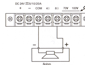
Connecting the speakers to 8 ohm output
